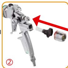
SATAjet 3000 B: insert the "dock" and slide in the "display"
